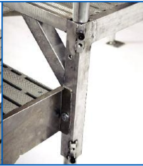
▲ Landing & Step Unit Fit Together with Simple Sleeve System
